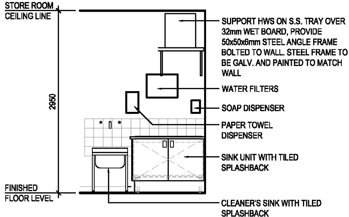
D ELEVATION A03WD SCALE 1:50 (A3)
